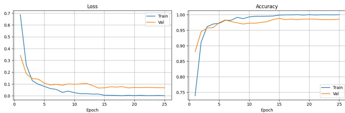
DeiT Model Training Metrics
