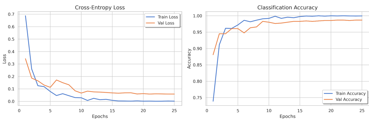
DeiT Model Training Metrics
